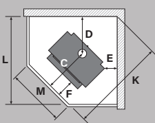
Corner clearances
