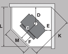
Corner clearances
